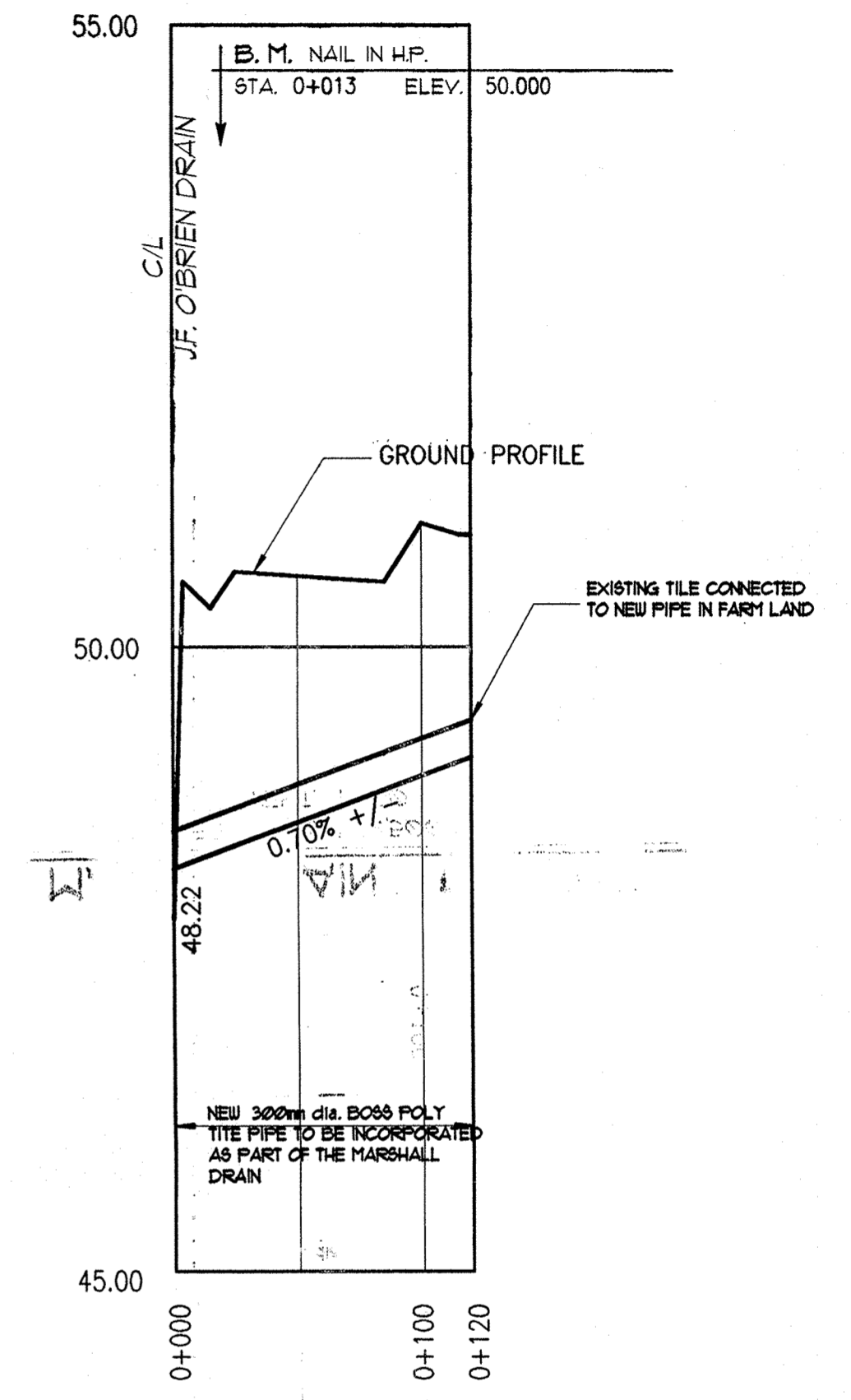
MAIN DRAIN PROFILE SCALE: HORIZ: 1:2500 VERT: 1:50
