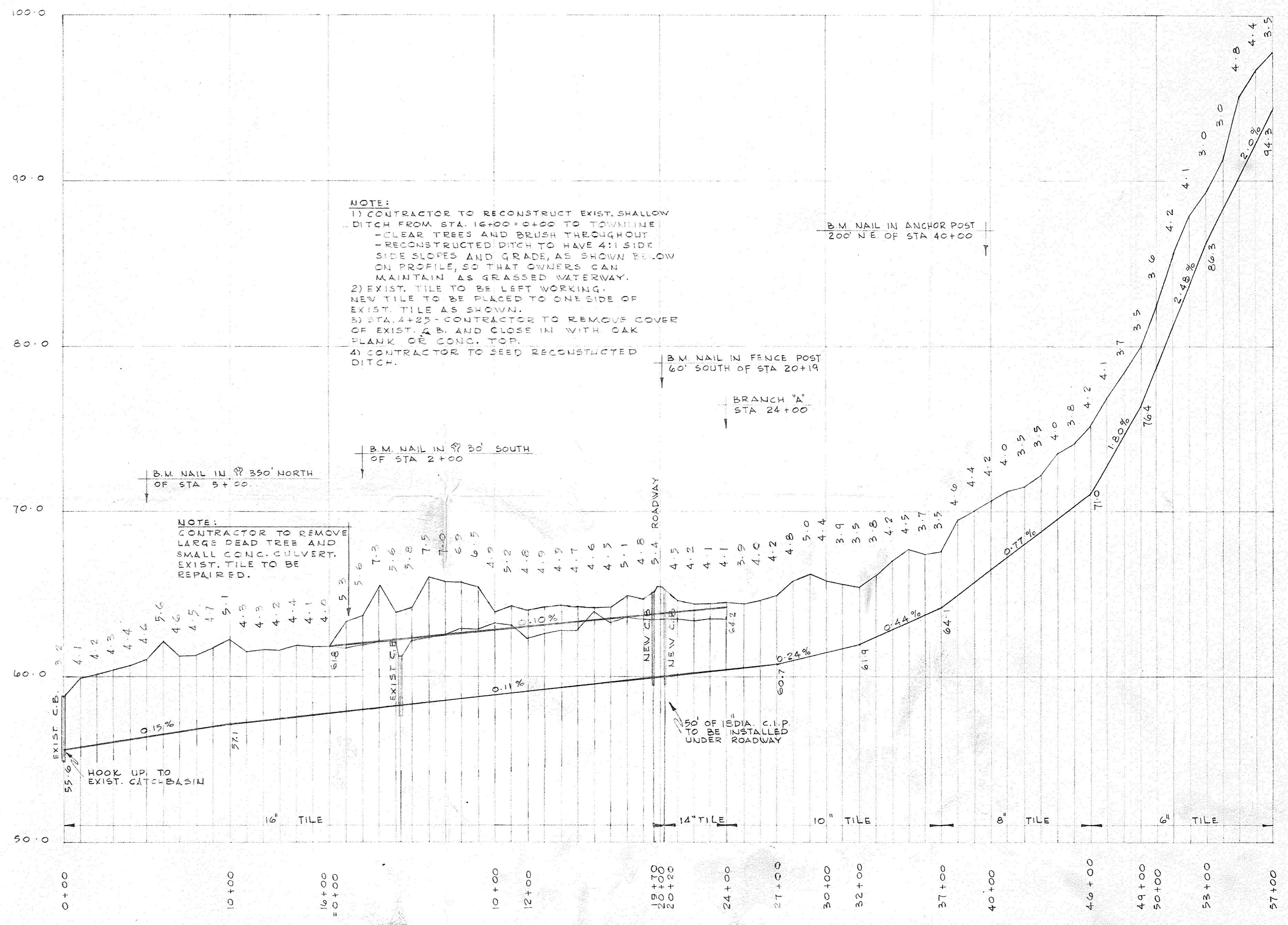
MAIN DRAIN PROFILE
